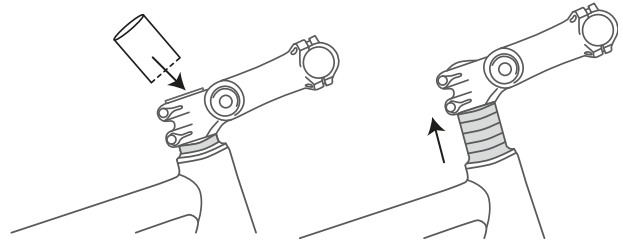
Figure 102: Raising the Ahead stem by fitting spacer rings
