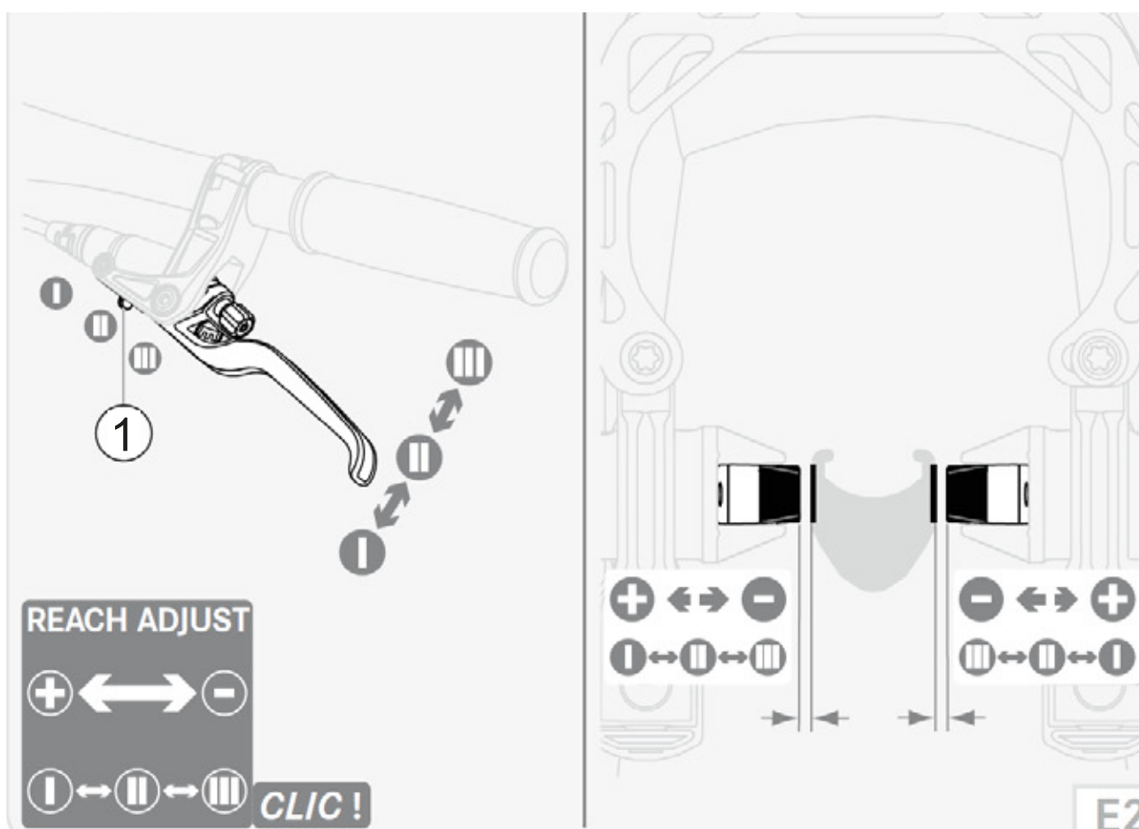
Figure 113: Setting the grip distance on a MAGURA HS 22 brake lever
