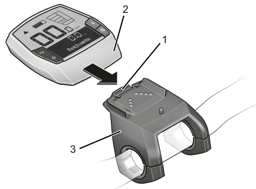
Figure 124: Push on-board computer (2) over the on-board computer catch (1) until it locks into the mount (3)
