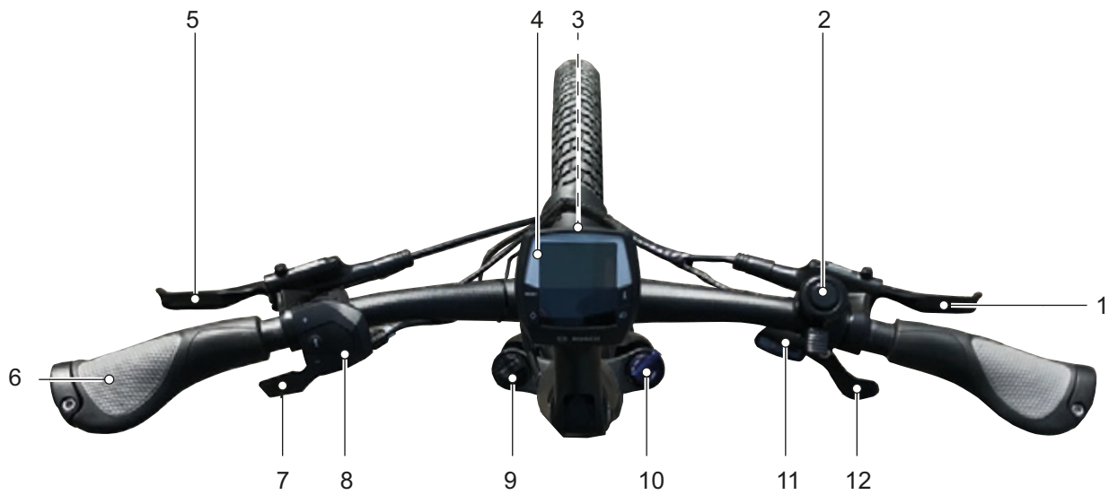
Figure 40: Detailed view of handlebars with BOSCH Intuvia on-board computer, example
