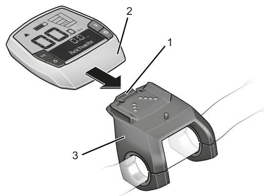
Figure 137: Push on-board computer (2) over the on-board computer catch (1) until it locks into the mount (3)
