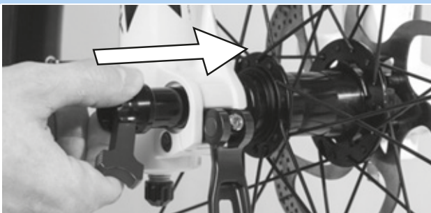
Figure 75: Inserting the cross axle in the direction of the arrow
