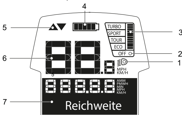
Figure 42: Overview of on-board computer display screen
