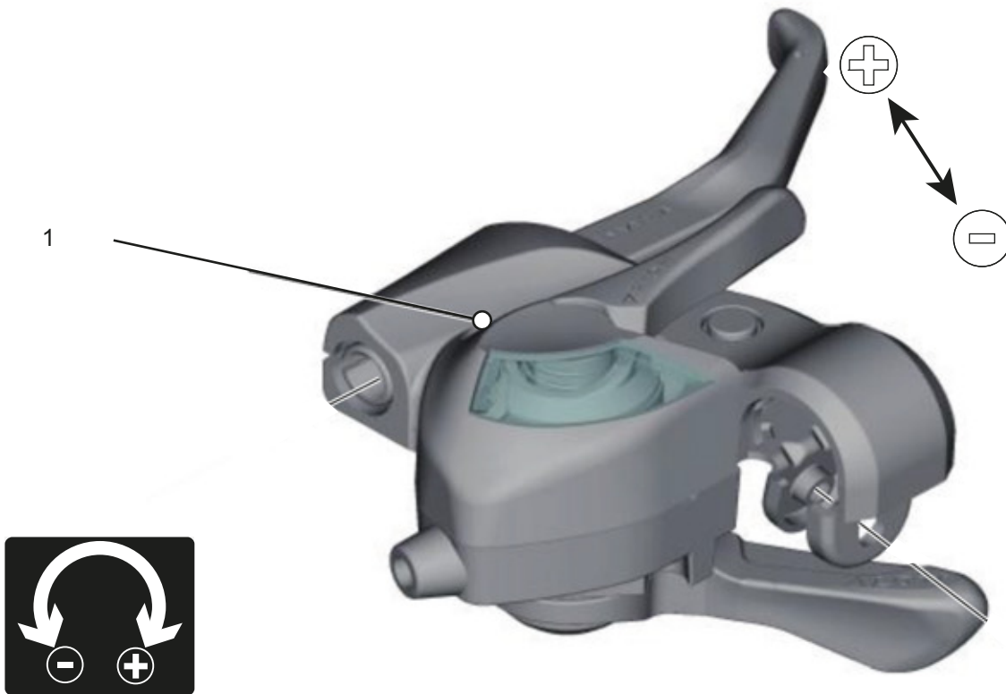
Figure 114: Setting screw position (1)
