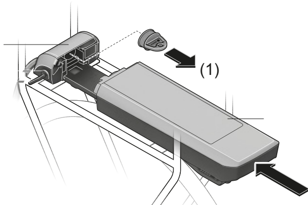
Figure 136: Covering open contacts with cover cap – example: pannier rack battery
