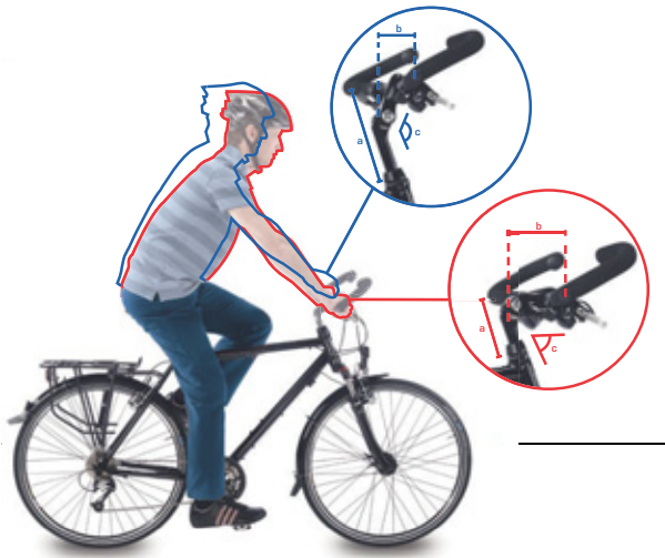
Figure 104: City bike (blue) and trekking bike position (red) by changing the angle
