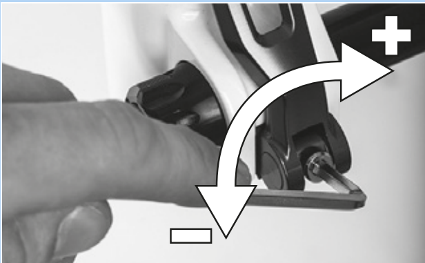
Figure 161: Adjusting the quick release clamping force
