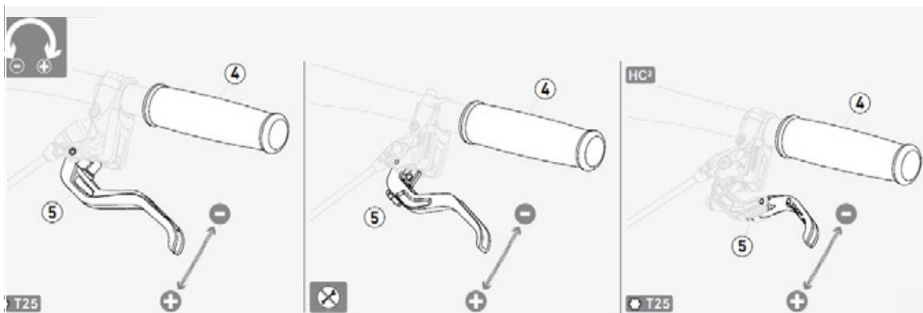
Figure 112: Adjusting the grip distance on a MAGURA disc brake lever
