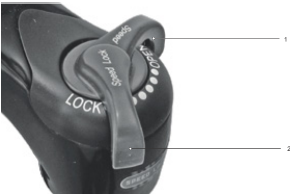
Figure 230: Changing compression adjuster to a harder setting
