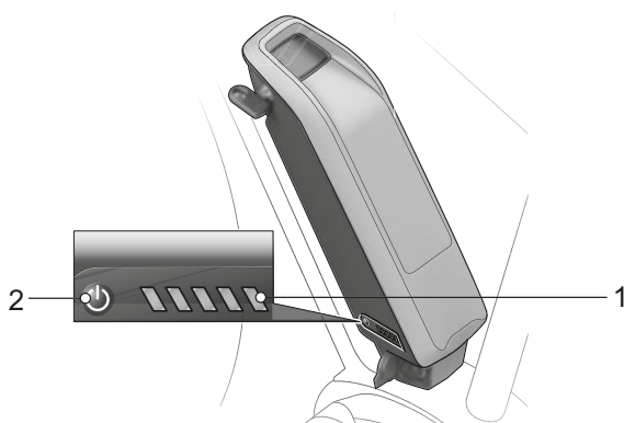
Figure 52: Position of charge level indicator on seat tube battery
