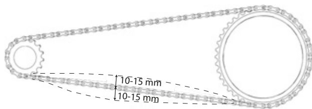
Figure 154: Checking the chain tension
