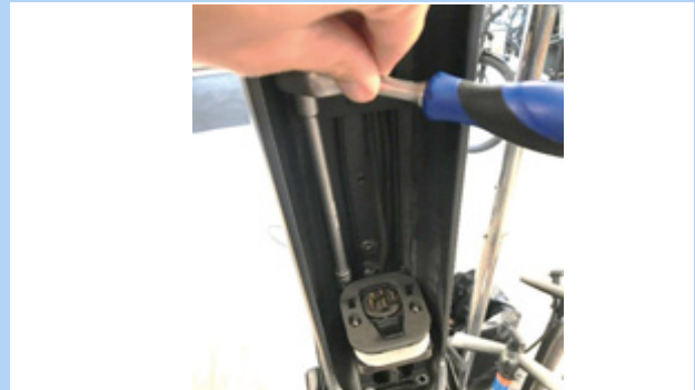
Figure 58: Removing hexagon screws
