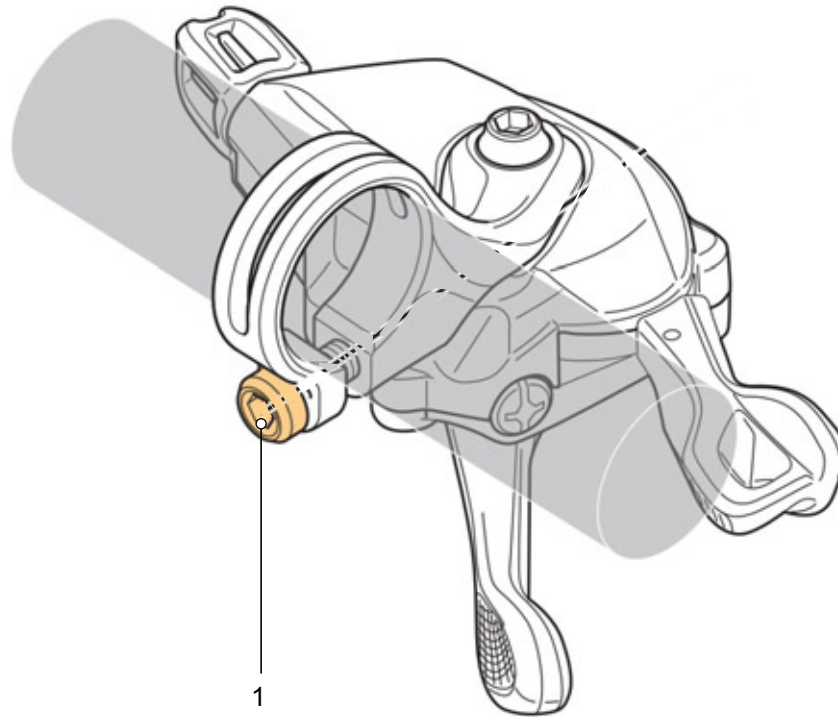
Figure 116: Position of attachment screw in SHIMANO shifter
