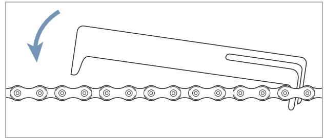
Figure 204: Lower gauge to the left
