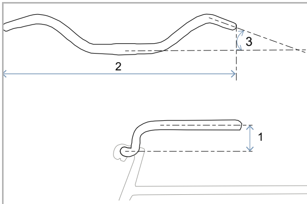
Figure 13: Handlebar dimensions
