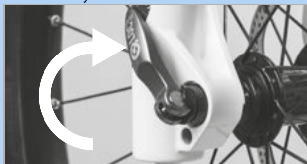
Figure 97: Closing the quick release
