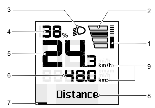
Figure 66: Overview of start screen
