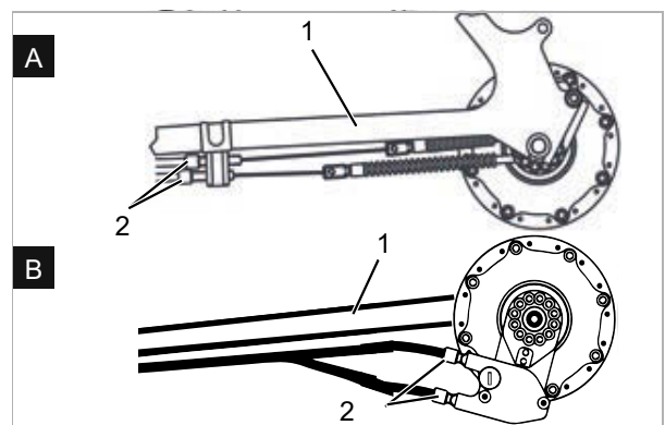
Figure 222: Adjusting sleeves (2) on two alternative versions (A and B) of a dual-cable, Bowden-cable-operated gear shift on the chain stay (1)
