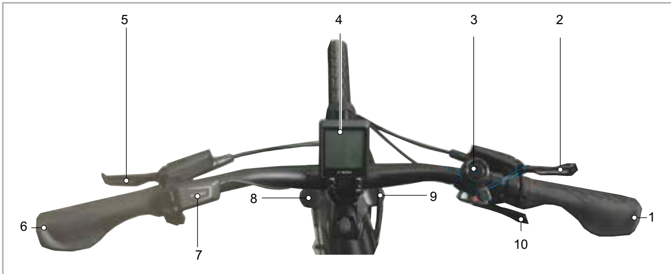
Figure 63: Detailed view of handlebars with BOSCH Intuvia 100 on-board computer, example
