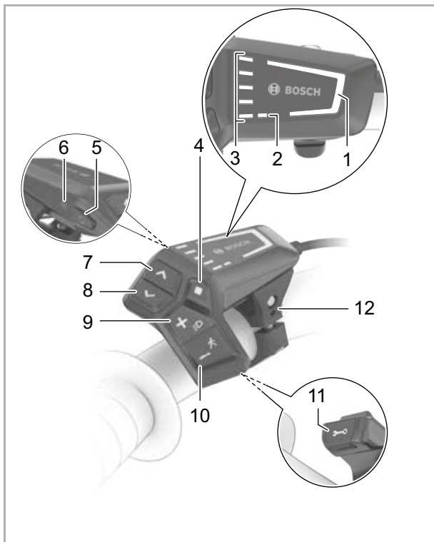
Figure 175: Overview of BOSCH LED Remote on-board computer
