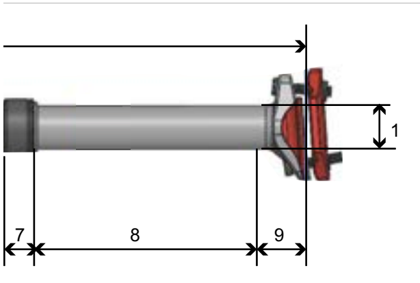
Figure 78: Dimensions of LIMOTEC A1 seat post
