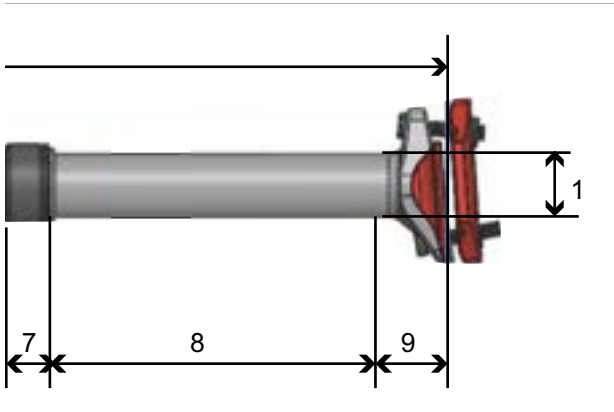
Figure 79: Dimensions of LIMOTEC A1L seat post
