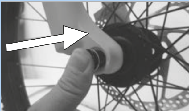
Figure 84: Inserting the axle in the direction of the arrow
