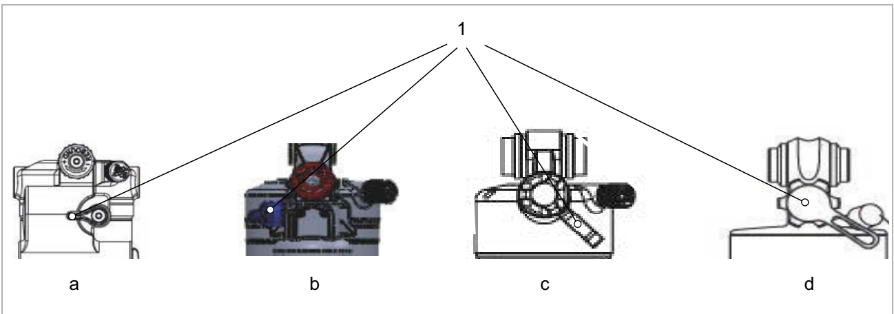
Figure 241: Position of RS Suntour compression lever for rear frame dampers Triair2 (a), Triair (b), EDGE-comp (c) and EDGE (d)
