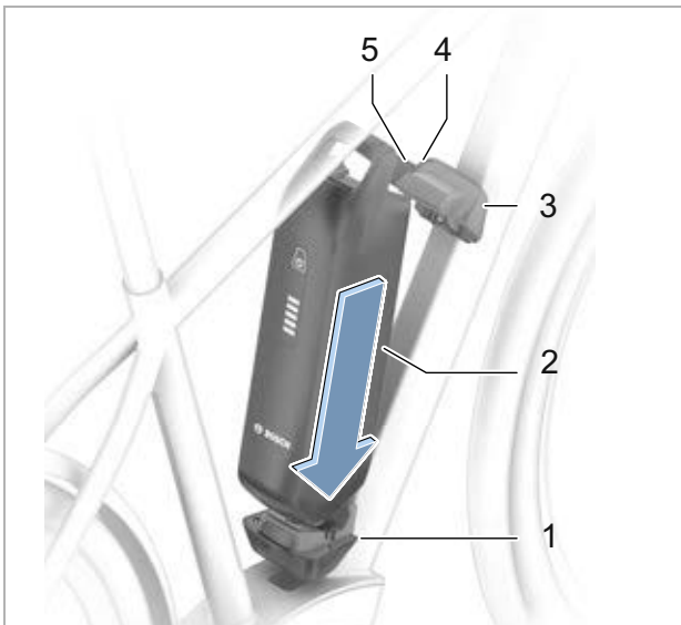
Figure 172: Inserting the PowerPack battery
