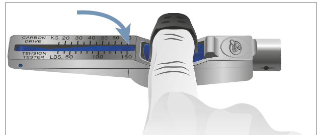
Figure 211: Index finger in the check gauge
