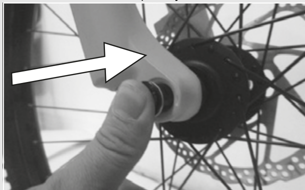
Figure 30: Fully inserting the axle
