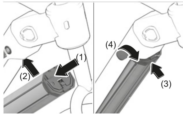
Figure 68: Inserting the integrated battery
