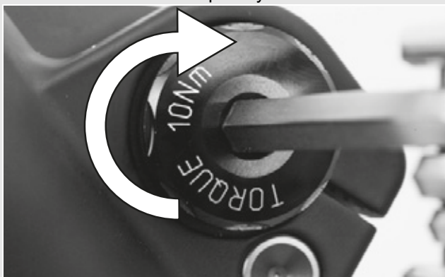
Figure 34: Tightening the inserted axle
