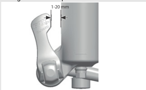
Figure 47: Spacing between lever and fork leg
