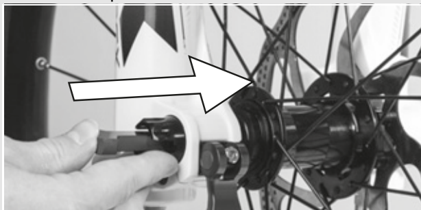
Figure 38: Pushing the quick release lever into the axle
