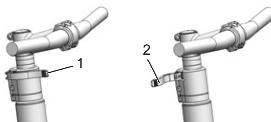
Figure 56: Open (2) and closed (1) stem clamping lever; All Up used as an example
