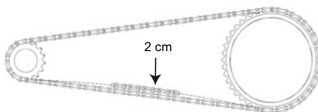
Figure 75: Checking the chain tension
