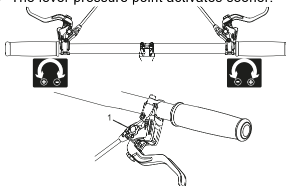
Figure 60: Using the twist knob (1) to adjust the pressure point
