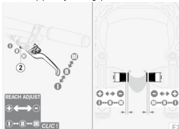
Figure 58: Setting the grip distance on a Magura HS 33 brake lever
