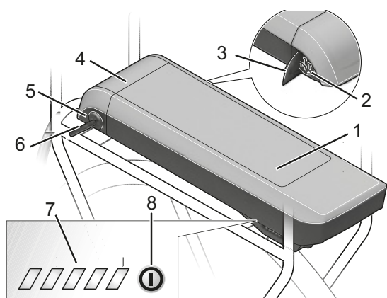
Figure 13: Details of pannier rack battery
