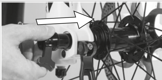
Figure 36: Pushing the axle into the hub
