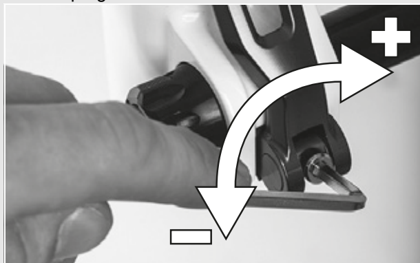
Figure 41: Adjusting the quick release clamping force
