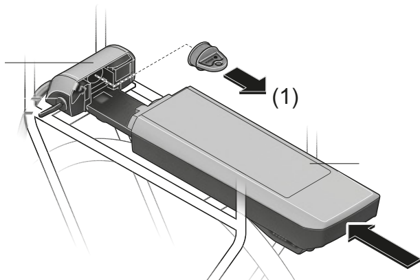
Figure 69: Covering open contacts with cover cap – example: pannier rack battery
