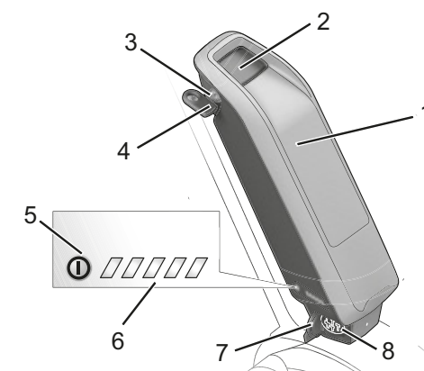
Figure 11: Details of frame battery
